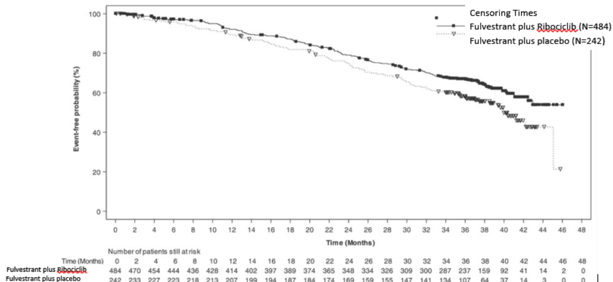
Figure 7: Kaplan-Meier plot of overall survival – MONALEESA-3 (Intent -to-Treat Population)
