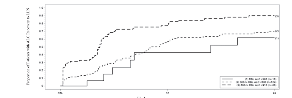
Figure 1: Kaplan-Meier Method; Proportion of Patients with Recovery to ≥ 910 cells/mm 3 LLN from the Recovery Baseline (RBL)
